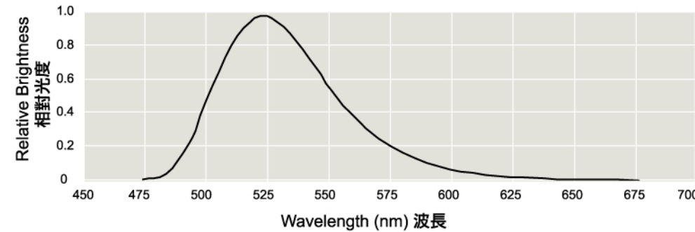
Fiber Spectrum at 80V/2000Hz 冷光纖光譜在 80伏/2000赫茲
