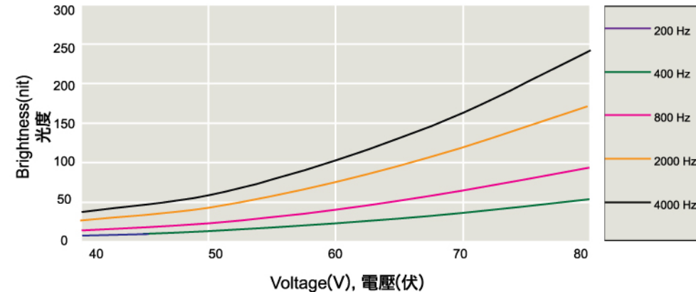
Typical Initial Reference Brightness 冷光纖始光度參考值
